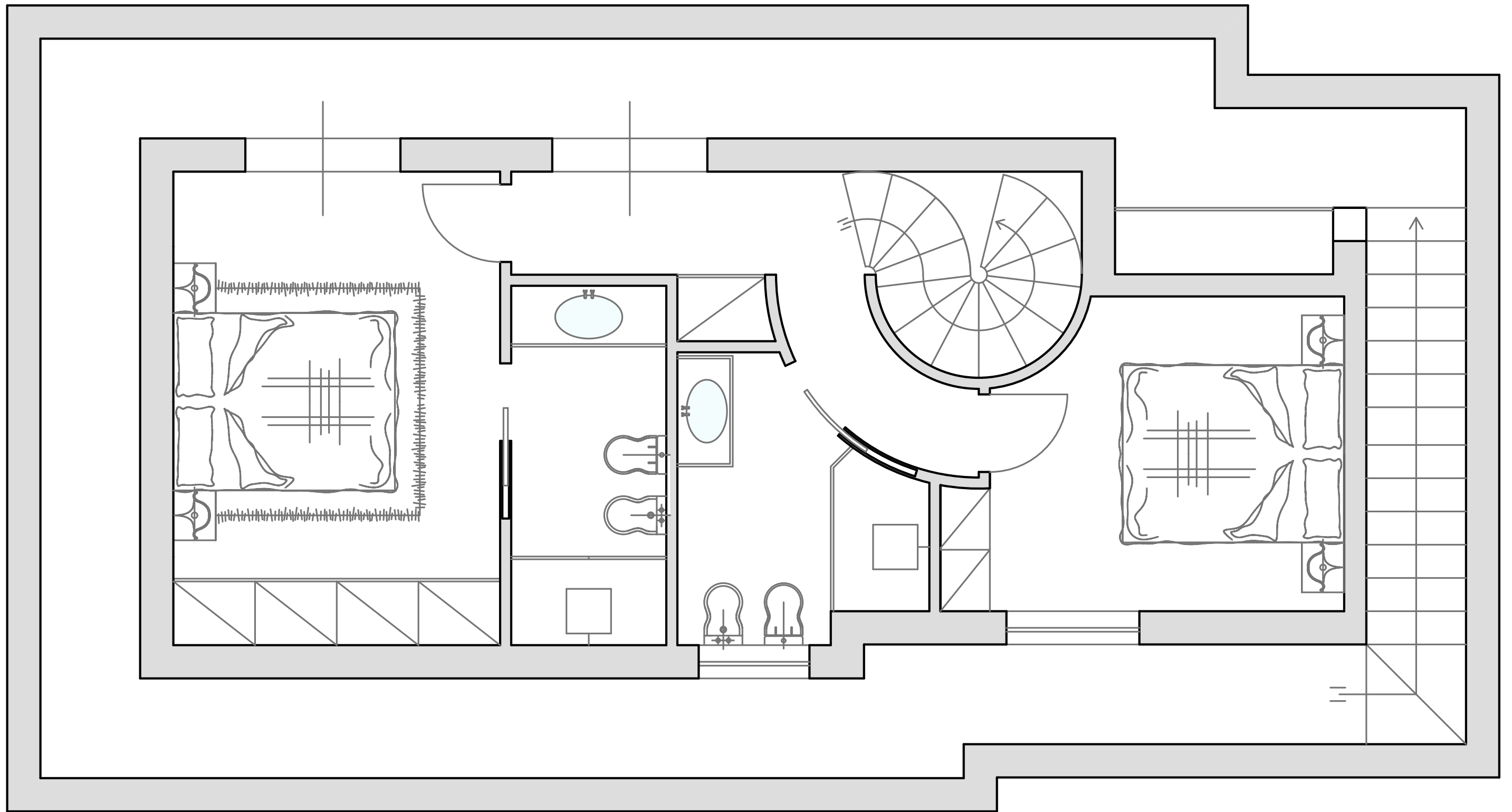
Piano Interrato
